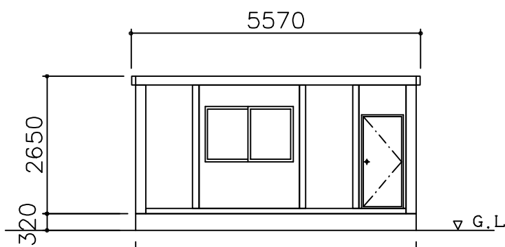
(Y0)通り立面図S=1/100
